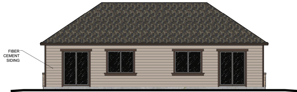
Rear Elevation Elevation C 1/4" = 1'-0"
