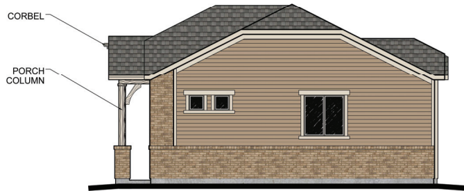
Right Elevation Elevation A 1/4" = 1'-0"
