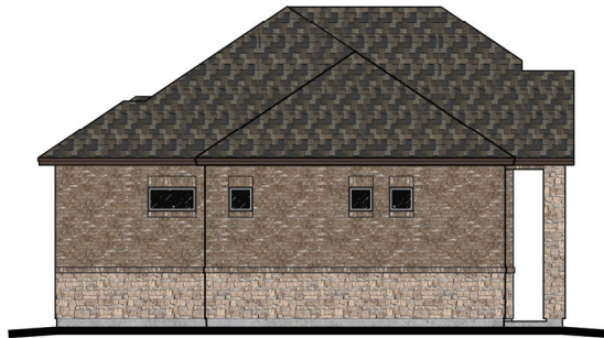
Left Elevation Elevation C 1/4" = 1'-0"
