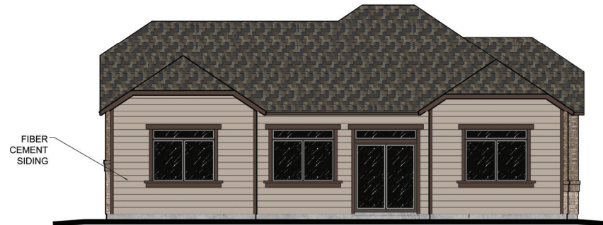
Rear Elevation Elevation C 1/4" = 1'-0"
