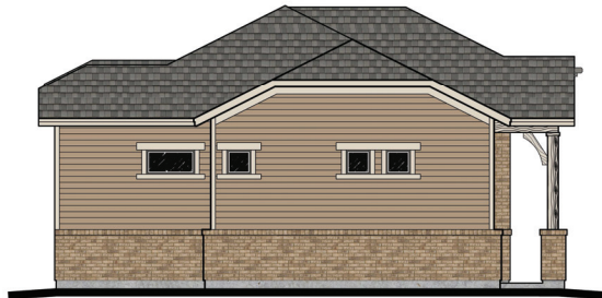
Left Elevation Elevation A 1/4" = 1'-0"
