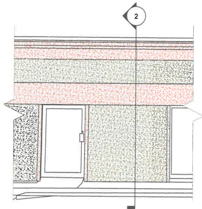
1 FRONT ELEV. NTS
