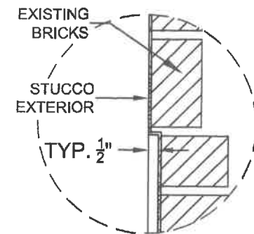
4 DETAIL SECT. NTS
