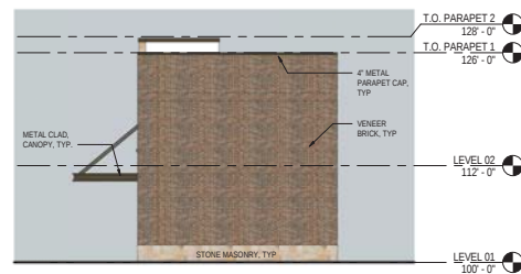
4 EXTERIOR ELEVATION - EAST 1/8" = 1'-0"
