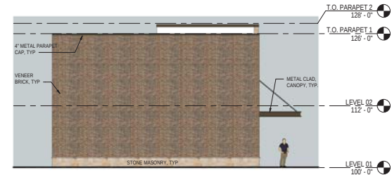
1 EXTERIOR ELEVATION - NORTH 1/8" = 1'-0"
