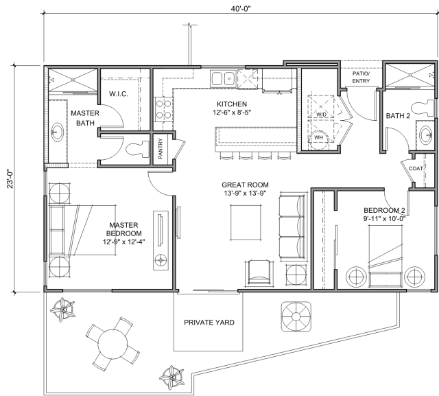
PLAN 2 - 2 BEDROOM 913 SF
