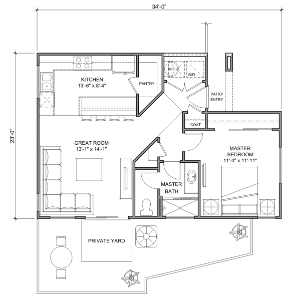
PLAN 1 - 1 BEDROOM 698 SF
