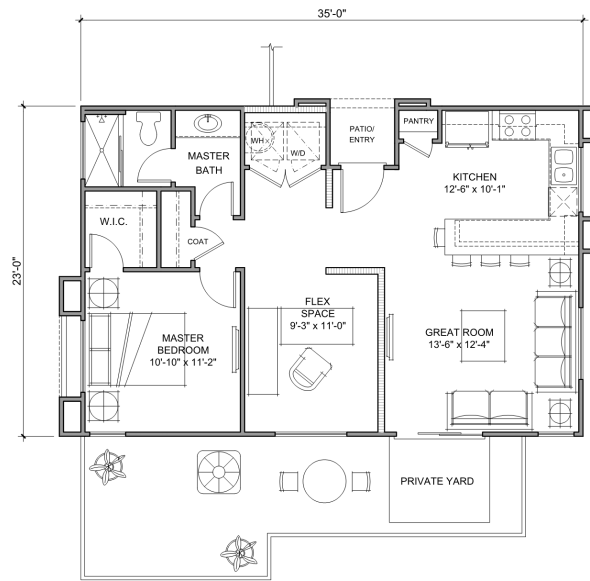
PLAN 1.5 - 1 BEDROOM + FLEX 786 SF
