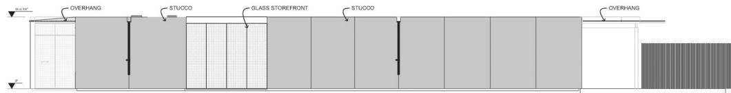
3 OFFICE EXTERIOR ELEVATION EAST SCALE: 1/8" = 1'-0"
