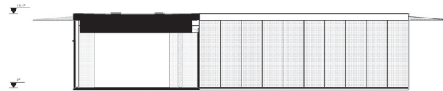
3 OFFICE EXTERIOR ELEVATION/SECTION COURTYARD EAST SCALE: 1/8" = 1'-0"
