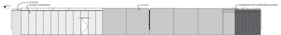
1 OFFICE EXTERIOR ELEVATION SOUTH SCALE: 1/8" = 1'-0"
