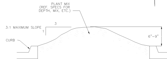
TYPICAL PARKING LOT ISLAND MOUNDING
