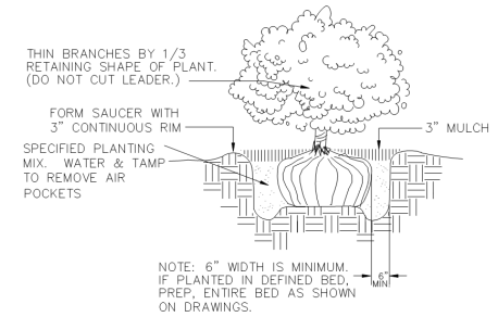
SHRUB PLANTING
