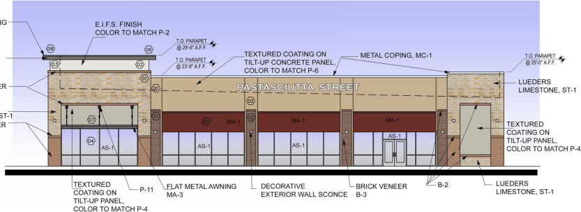
02 SOUTH ELEVATION (RETAIL B)
