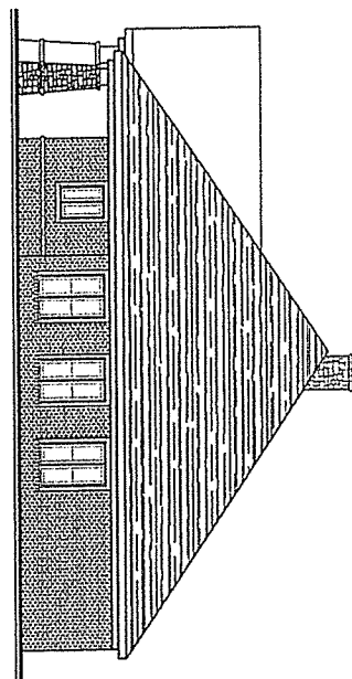
NORTH ELEVATION
