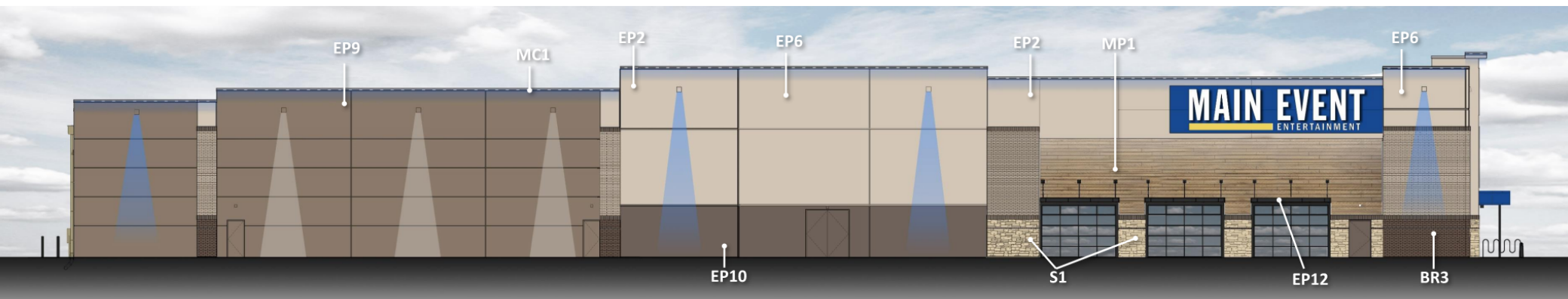
SOUTH ELEVATION
