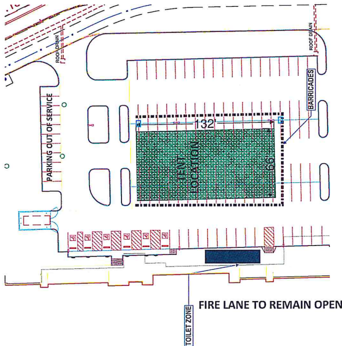
VICINITY PLAN
